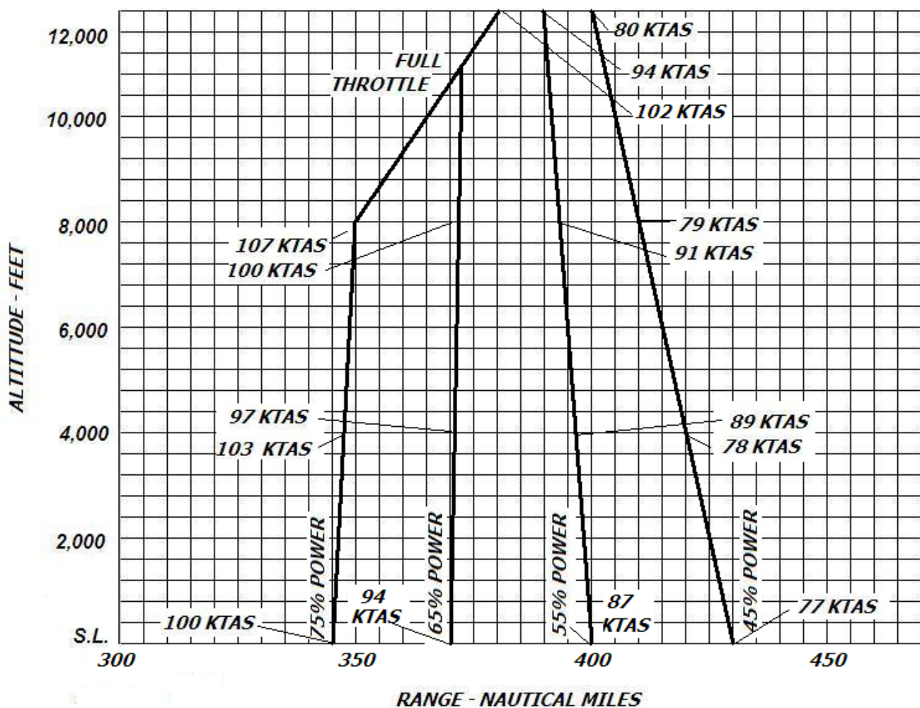
Figure 5-8 Range Profile (Sheet 1 of 2)
