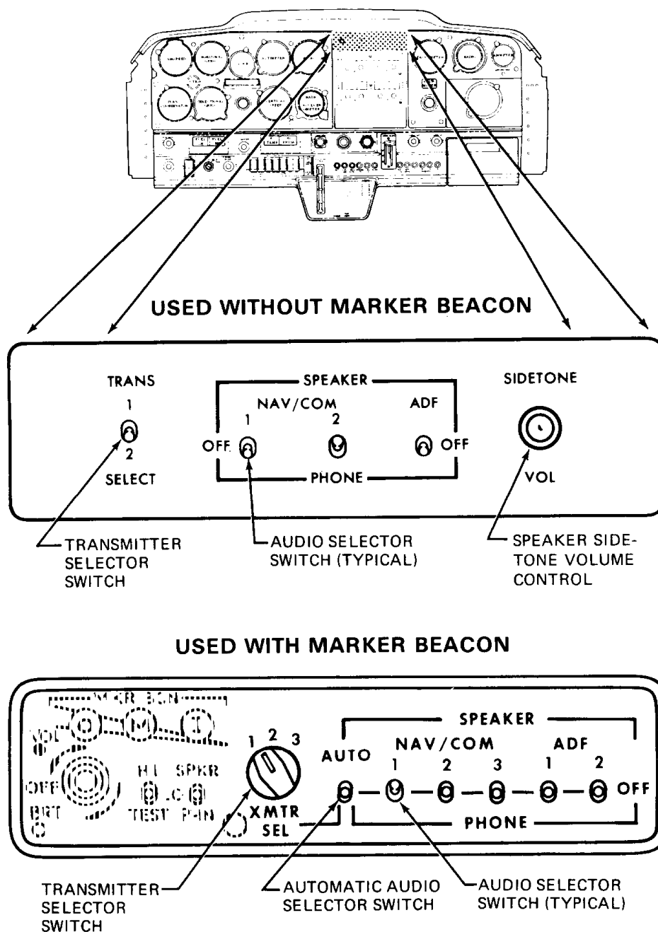
Figure 7-10. Audio Control Panel
