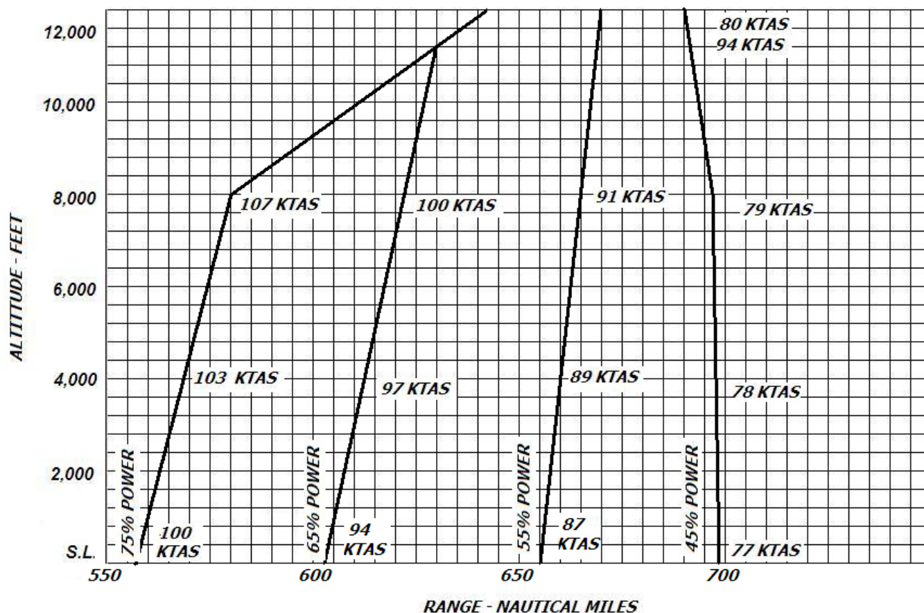
Figure 5-8 Range Profile Sheet 2 of 2)
