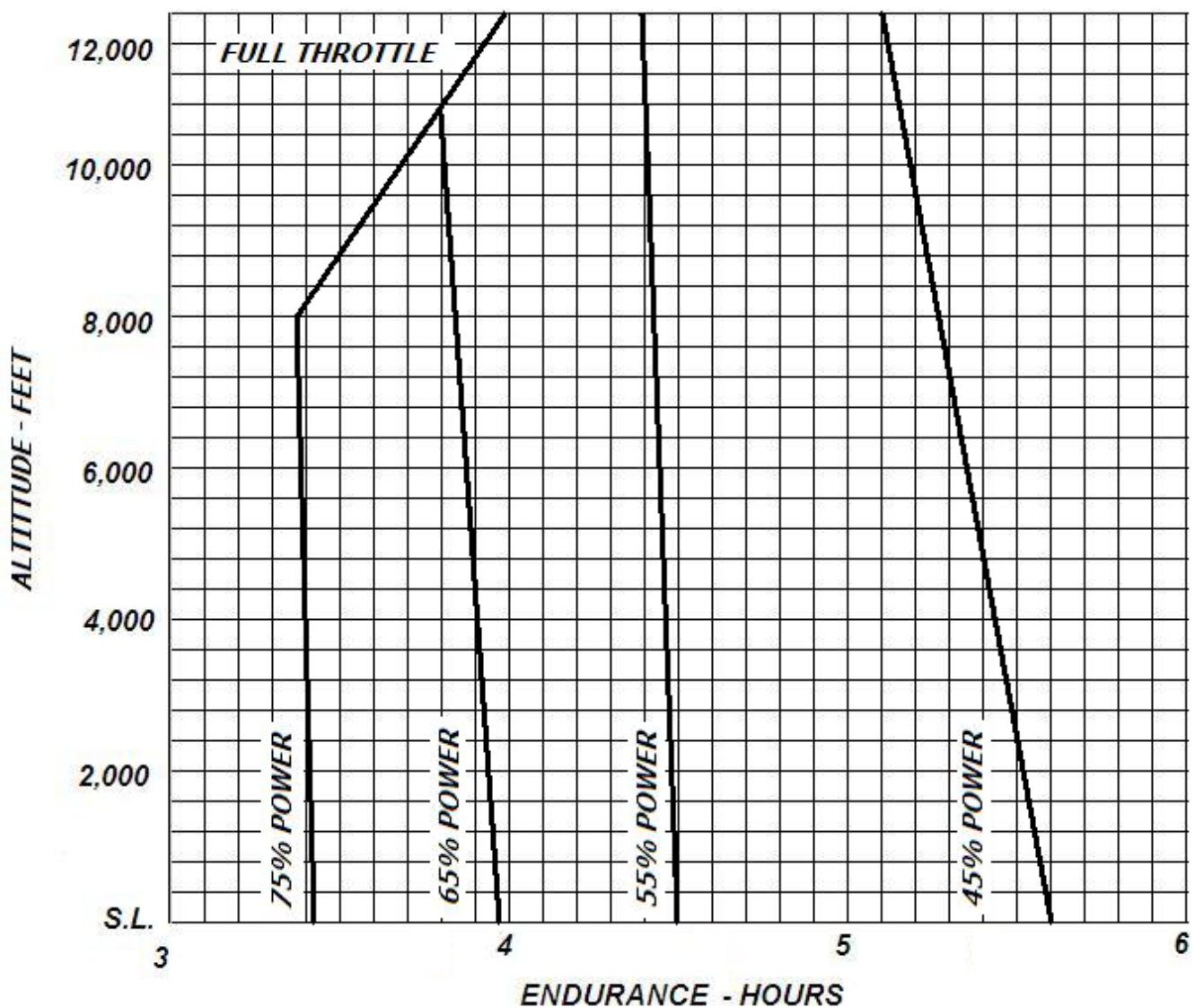
Figure 5-9 Endurance Profile (Sheet 1 or 2)
