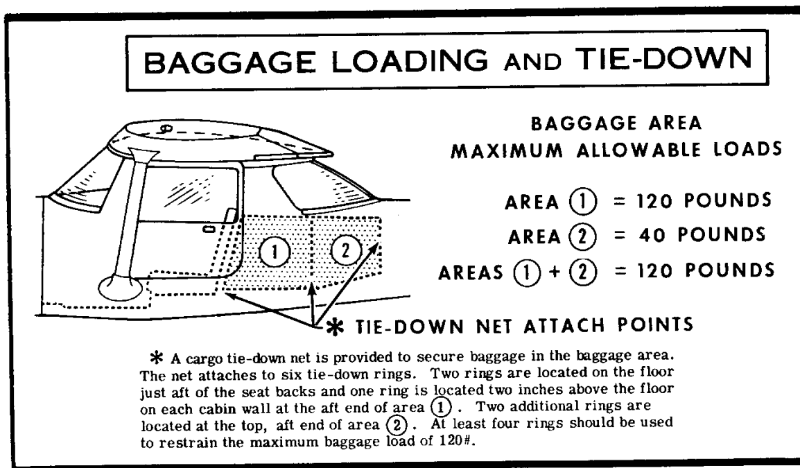
Figure 6-4. Baggage Loading and Tie-Down
