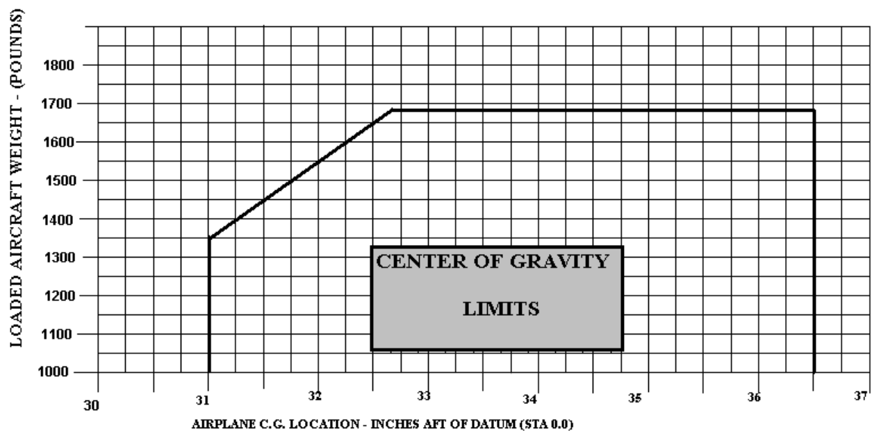
Figure 6-9 Center of Gravity Limits
