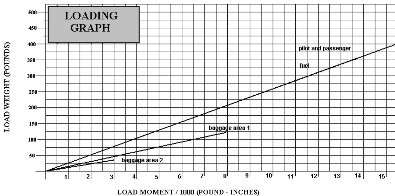
Figure 6-7 Loading Graph
