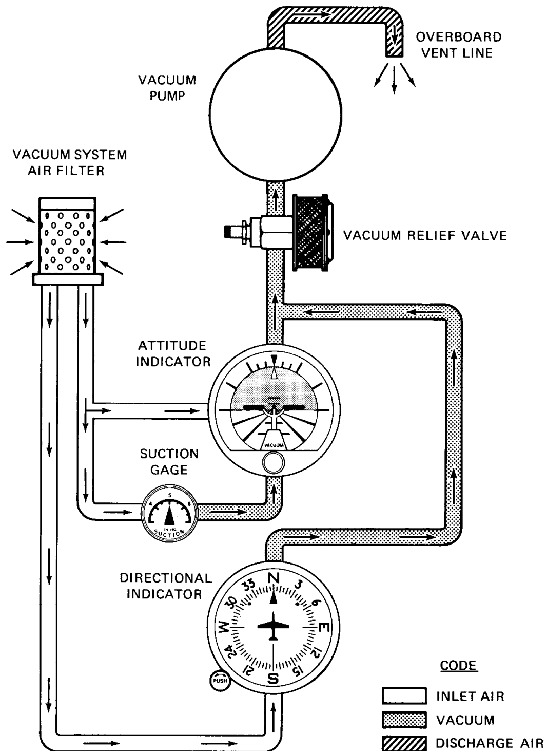
Figure 7-9. Vacuum System
