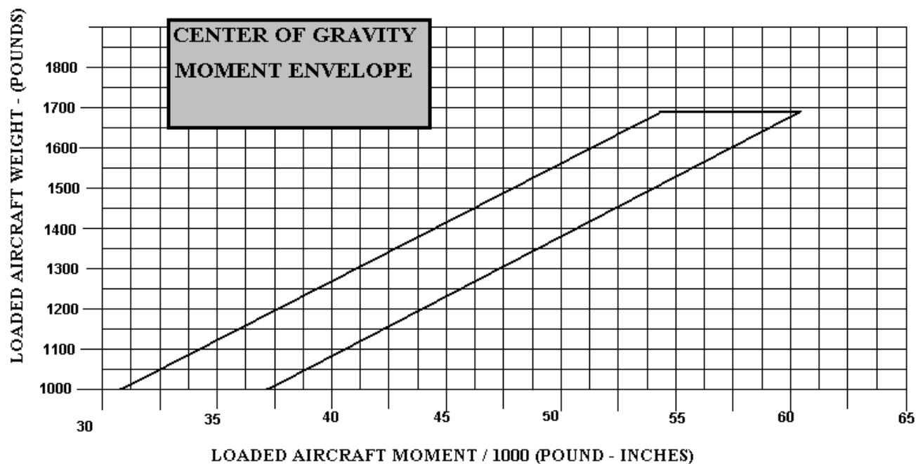
Figure 6-8 Center of Gravity Moment Envelope
