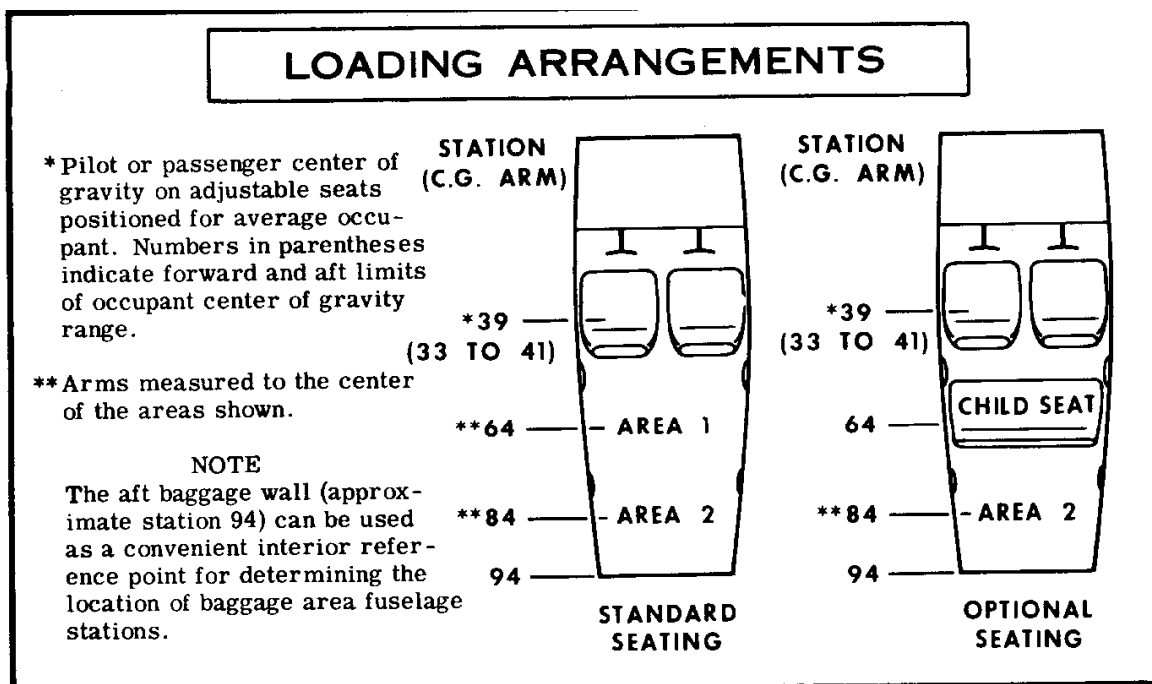
Figure 6-3. Loading Arrangements
