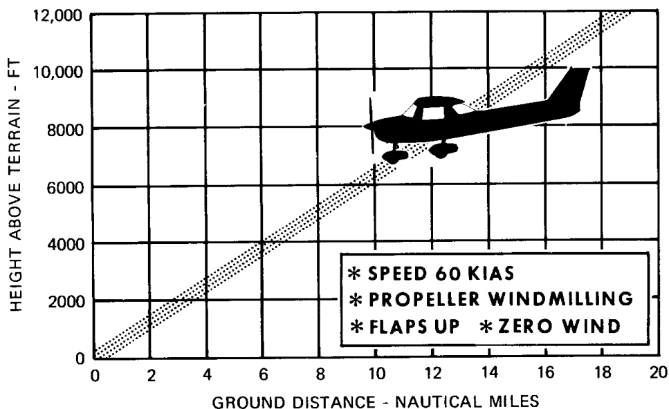
Figure 3-1. Maximum Glide
