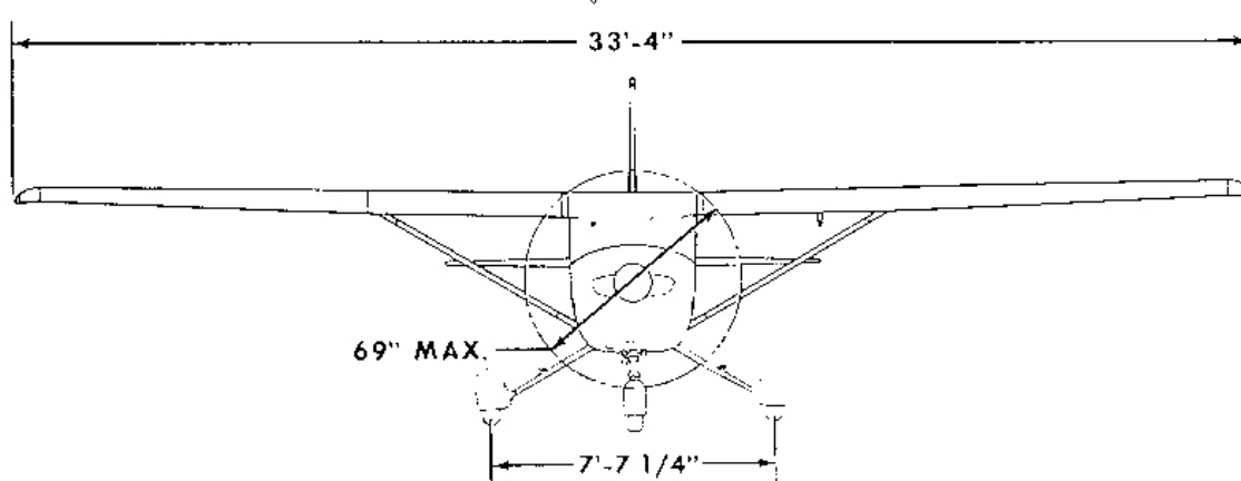
Figure 1-1 Three View
