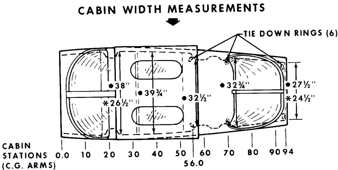
Figure 6-5. Internal Cabin Dimensions
