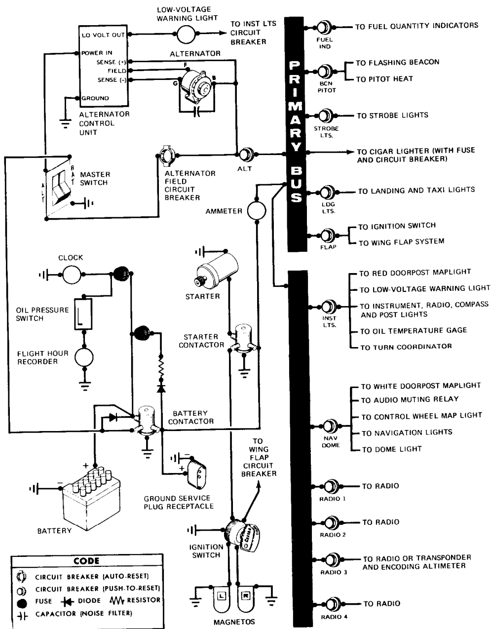
Figure 7-7. Electrical System
